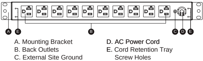
Back View
